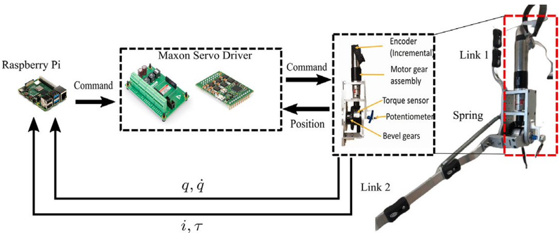
Figure 5. The 1-DOF knee exoskeleton used in the experimental study, including the Raspberry Pi for the implementation of the closed-loop control and the Maxon servo drivers for issuing motor commands.
