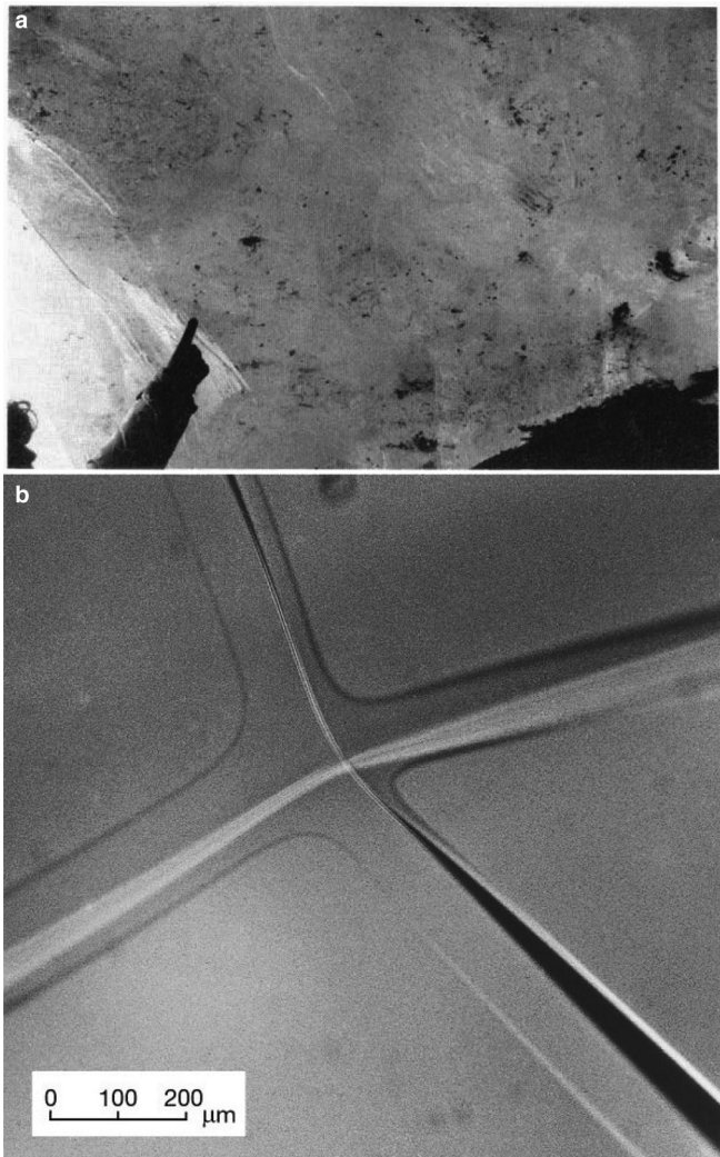
Figure 1. (a) Photograph showing diffuse debris in basal ice near Kangerlussuaq, Greenland (reproduced with permission from Knight and Knight, 1994). (b) Photograph of four veins meeting at a node to form a connected network through polycrystalline ice (provided by Heidy Mader; see Mader, 1992a). Note that the center of curvature for each of the vein walls is inside one of the four ice grains depicted so that vein cross-sections more closely resemble triangles than circles, with optical interference producing brightening along the middle (third) edges of the two sub-horizontal veins and darkening on the middle edges of the two sub-vertical veins shown here.
