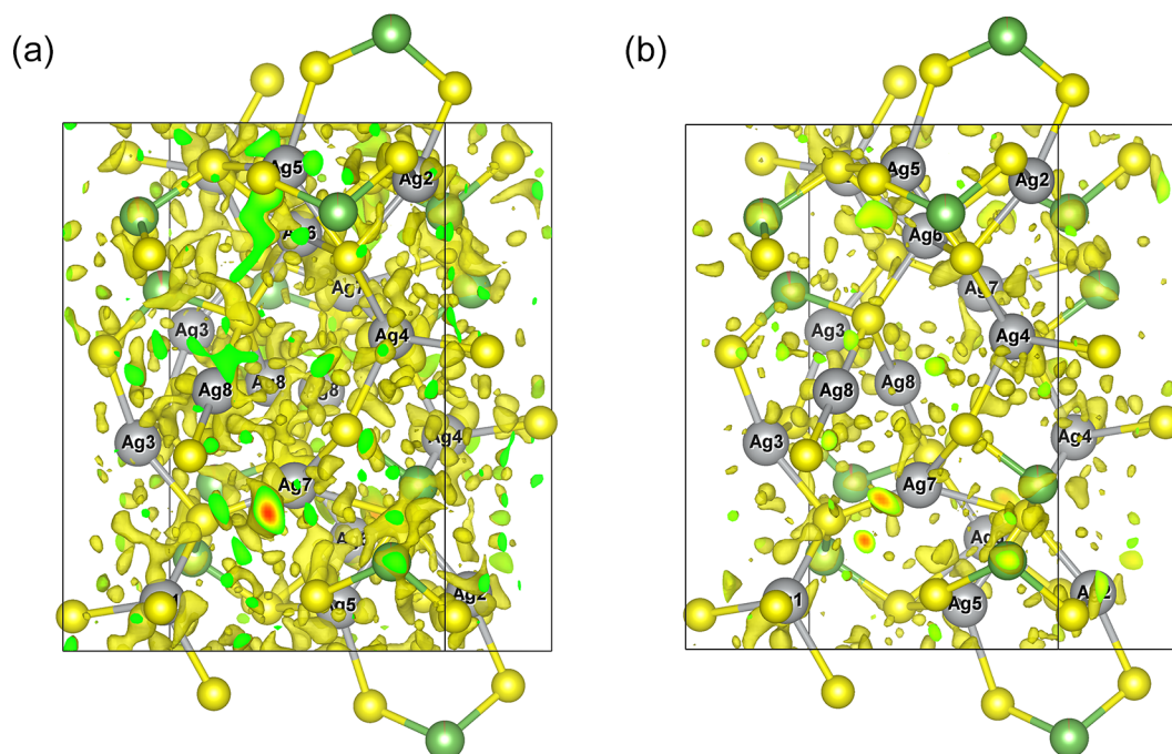
Figure 7. Difference-Fourier 3D maps plotted for the entire unit cell of derpillite. (a) Harmonic vs. (b) non-harmonic refinement. The isosurface level is set to the same value (0.25).
