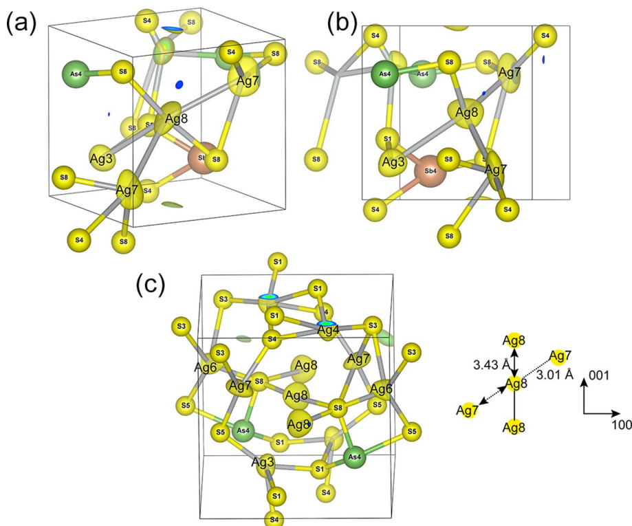
Figure 8. Three different projections providing a view of the non-harmonic atomic displacement parameters of Ag in the structure of derpillite (represented by the j.p.d.f. isosurface). The metal-metal interactions are displayed as dark-grey joins, and the size of the S, As/Sb atoms is set arbitrarily. Noteworthy is a pseudo-linear arrangement of the Ag8-Ag8 atoms in the structure (extending along c) and 'diagonally' arranged interacting Ag7 atoms (approximately in a plane). The highest mobility of the silver (diffusion) could be expected there at non-ambient temperatures. The j.p.d.f. calculations by Jana2020 and plotted by Vesta3 . The isosurface level of the 3D maps is 0.05 \text{ \AA}^{-3} .
