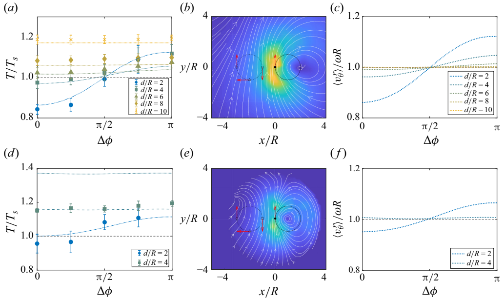
Figure 4. Hydrodynamic interactions between rotating helices under confinement ( a–c ) R_0 = 7R and ( d–f ) R_0 = 3.5R . ( a, d ) Torque on one helix in the helical pair as a function of phase difference \Delta\phi at different spacings d . Symbols denote experimental data, while dotted lines represent model predictions (3.2). The green dashed line in ( d ) is the model prediction using experimentally obtained T_e/T_c , instead of (3.1). ( b, e ) Flow field in the x - y plane of a rotating helix positioned at (R, 0) . The circle on the right indicates the helix's trajectory, while the dashed circle on the left represents the trajectory of an imaginary helix. Three phase differences between the real helix and the imaginary helix are shown, consistent with those in figure 3( a ). ( c, f ) Velocity of the imaginary helix in the reference frame of local flow, \langle v_\theta^r \rangle , normalised by the helix's rotation speed in the lab frame, \omega R , as a function of \Delta\phi at different d .
