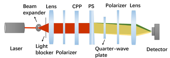
Figure 5. Setup to measure the polarization distribution in the far field using a rotating quarter-wave plate.
